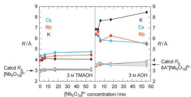
Figure 2. Variation of radii ( R_g , R_s , R_{ss} ) with solution concentrations of A_8[Nb_6O_{19}] \cdot xH_2O ( A = K, Rb, Cs ) in 3 M TMAOH (left panel) and 3 M AOH (right panel). The Guinier radii of gyration R_g are shown as open symbols connected with dashed lines. The solid sphere radii R_s obtained by fitting the SAXS obtained in 3 M TMAOH with a solid sphere form factor are shown in the left panel as filled symbols connected with solid lines. The spherical shell radii, R_{ss} , obtained by fitting the SAXS obtained in 3 M AOH with a spherical shell form factor are shown in the right panel as filled symbols connected with solid lines. The calculated R_g values for bare [Nb_6O_{19}]^{8-} and A_8[Nb_6O_{19}] are indicated with arrows in the left and right panels, respectively.
